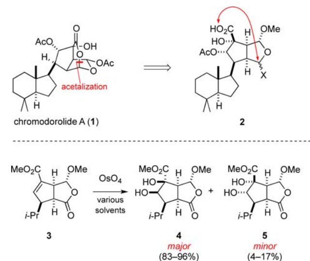
Figure 1. Structure of chromodorolide A ( 1 ) and experimental results of dihydroxylation of cis -oxabicyclo[3.3.0]octenone 3 .
