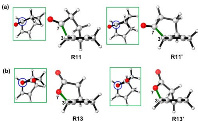
Figure 8. Optimized structures of (a) R11 and R11' and (b) R13 and R13'.
