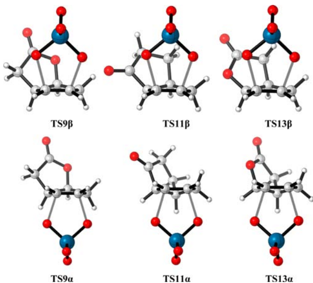
Figure 6. Optimized \beta - and \alpha -dihydroxylation transition structures of cis -bicyclo[3.3.0]octenes 9 , 11 , and 13 .
