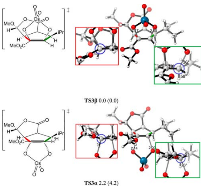
Figure 2. Optimized \beta - and \alpha -dihydroxylation transition structures of cis -oxabicyclo[3.3.0]octenone 3. The Newman projections of interest shown in the red and green box insets are viewed along the red and green bonds, respectively. Values below each structure are relative energies in kcal/mol calculated by B3LYP. Values enclosed in parentheses are relative energies in kcal/mol calculated by B3LYP-D3.
