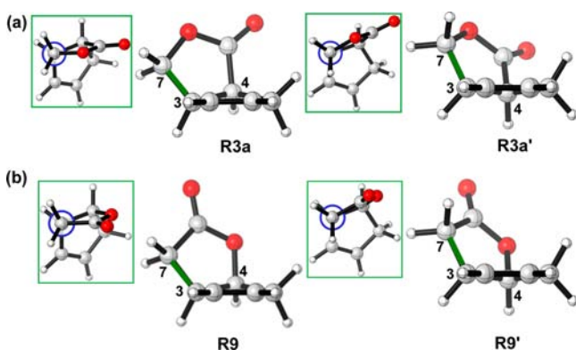
Figure 7. Optimized structures of (a) R3a and R3a' and (b) R9 and R9'.
