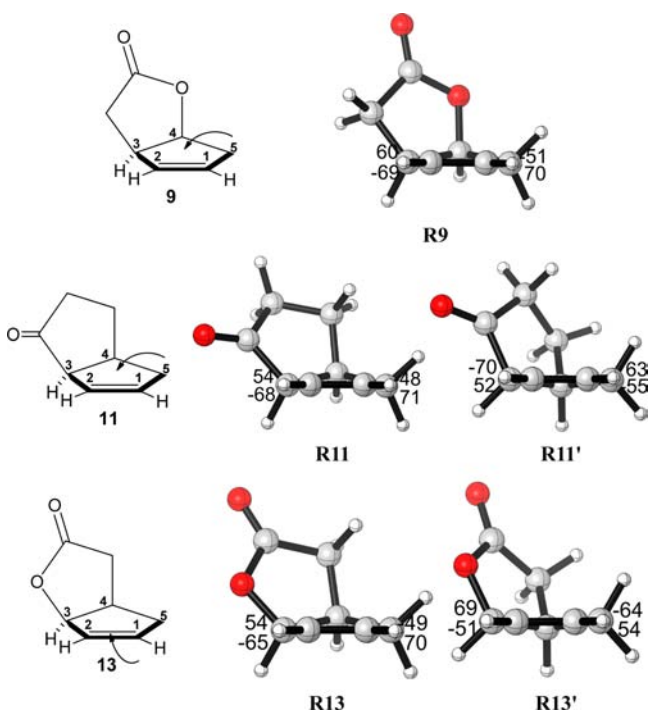
Figure 5. Three fused cyclopentene compounds and their optimized geometries. In R9 , R11 , and R13 , the flap of the envelope is up; in R11' and R13' , it is down.
